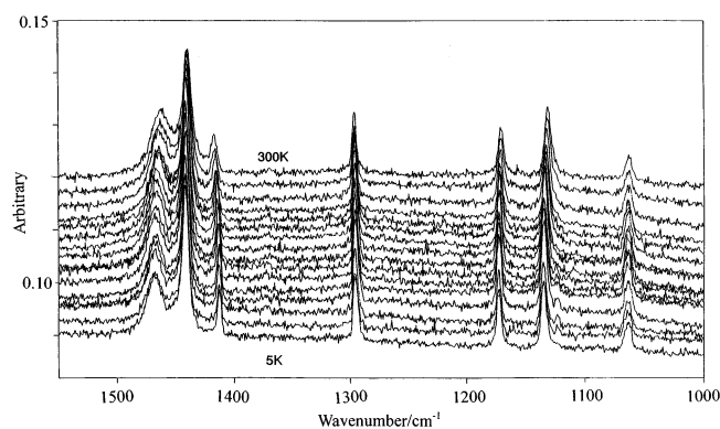
Figure 4. (a) Raman spectra of polyethylene in the temperature region 5–300 K.
